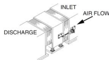
TYPICAL FAN HEAD
