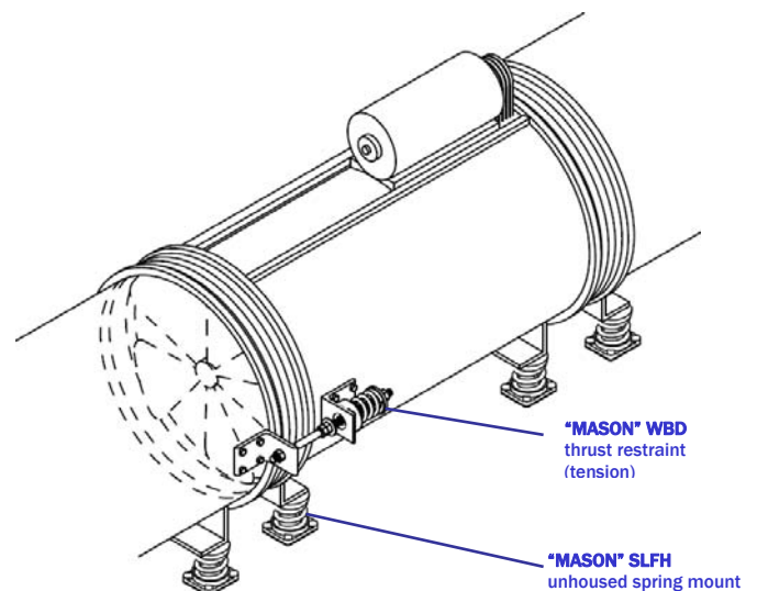
Typical Vibration Isolation measures at tunnel fan head
